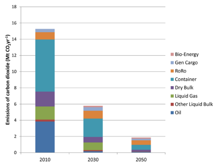
Figure 20: Levels of annual CO 2 emissions associated with UK imports in 2010, 2030 and 2050 in the S2 scenario.
