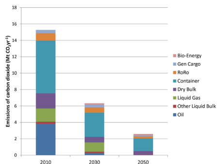
Figure 24: Levels of annual CO 2 emissions associated with UK imports in 2010, 2030 and 2050 in the S3 scenario.
