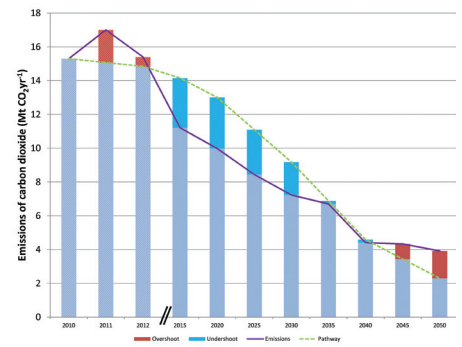
Figure 18: Annual and cumulative CO 2 emissions from the baseline year out to 2050 in the S1 scenario.
